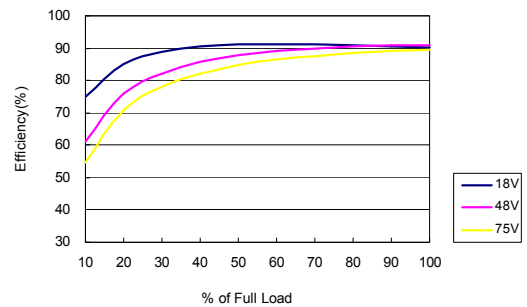
MJWI25-48S05 Efficiency vs Load Current
