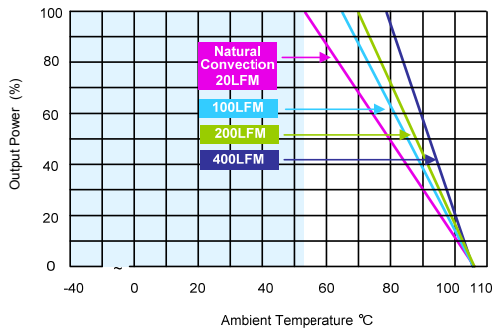
MJWI25-24S033 Derating Curve without Heatsink
