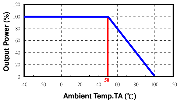
Power Derating Curve (Without Heatsink)
