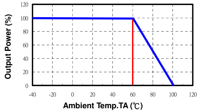
Power Derating Curve (With Heatsink)
