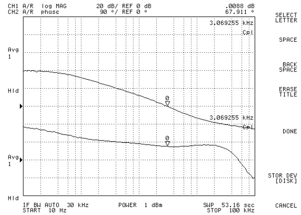
Loop Gain & Phase at Vi=48V, Full Load
