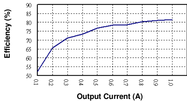
BOA5-48S1 Output Current vs. Efficiency
