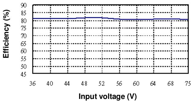
BOA5-48S1 Input voltage vs. Efficiency
