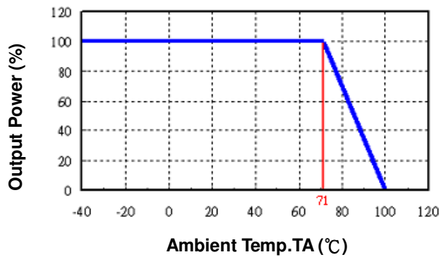
BOA5 Series Power Derating Curve(4)
