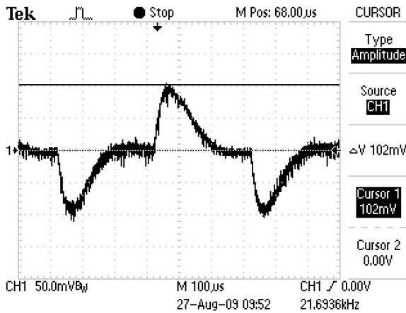
Transient Response at 50%~100% Max Load
