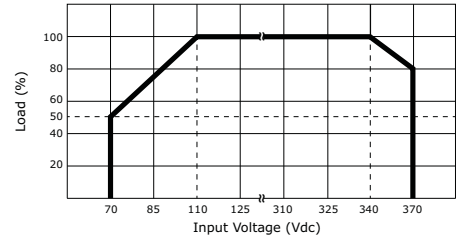
3. output power vs. input voltage [Vdc]
