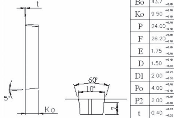
Figure 19 – VPOL20A-12W-SMT Tape and Reel Dimensions
