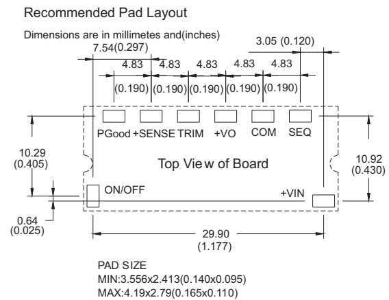
Figure 8. Recommended VPOL10A-12W-SMT Footprint
