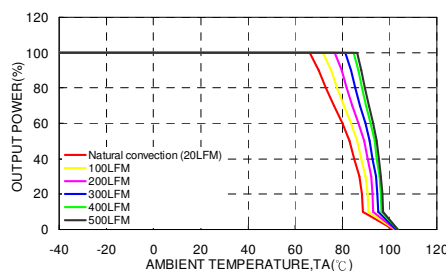
HAE100-48S05W Derating Curve (Note 2) With 0.24" Height Heat-sink
