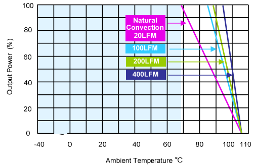
MKWI50-24S033, MKWI50-48S033 Derating Curve with Heatsink
