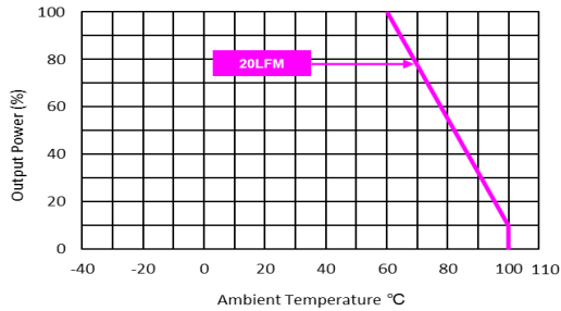
MJWI30-24S05, MJWI30-24S12, MJWI30-24S15, MJWI30-24S24 MJWI30-24D12, MJWI30-24D15, MJWI30-48S05 Derating Curve without Heatsink
