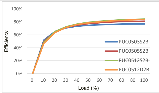
PUC05-2B Efficiency vs. load current at T_{P1} = +25^{\circ}\text{C} .
