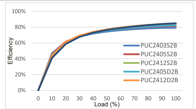
PUC24-2B Efficiency vs. load current at T_{P1} = +25^{\circ}\text{C} .
