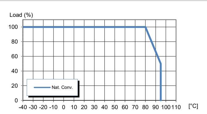
Available load vs. ambient air temperature. See Thermal Consideration section. (others)
