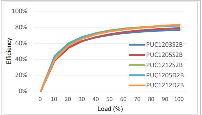
PUC12-2B Efficiency vs. load current at T_{P1} = +25^{\circ}\text{C} .
