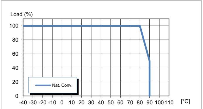
Available load vs. ambient air temperature. See Thermal Consideration section. (PUC1212S2B and PUC1212D2B)
