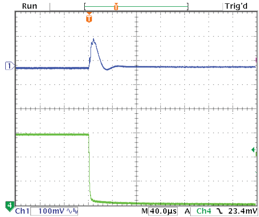
Step Load Transient Response (Vin=5.5V, Vout=3.3V, Cload=10x10µF X5R 0805 ceramic, plus 1x470µF, 7mΩ POSCAP, total 570µF, Iout=3A to 0A) Top trace=Vout, Bottom trace=Iout
