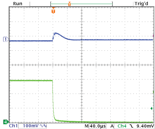
Step Load Transient Response (Vin=12V, Vout=3.3V, Cload=10x10µF 5R 0805 ceramic, plus 1x470µF, 7mΩ POSCAP, total 570µF, Iout=3A to 0A) Top trace=Vout, Bottom trace=Iout
